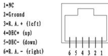
Figure 4. ST-4 Compatible Guiding Port Wiring
